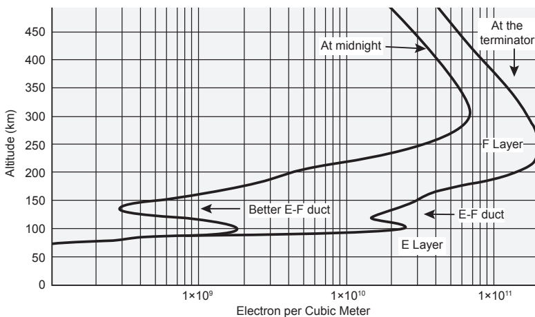
Figure 7 — The duct between the E and F layers of the ionosphere. Note the more pronounced duct at midnight, compared to the duct at the terminator. [Adapted from Robert R. Brown, NM7M, "On the SSW Path and 160-Meter Propagation," QEX, Nov/Dec 2000, pp. 3-9, Figure 1.]
