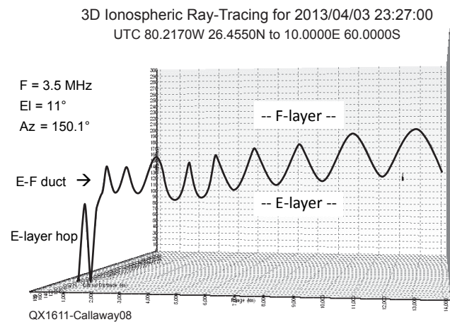
Figure 8 — A PropLab Pro 3.0 simulation of propagation in the E-F duct at the date and time of the N4BRF QSO with VK9CZ. The signal leaves N4BRF, makes one conventional E-layer hop, then enters the E-F duct, traveling more than 14,000 km.
