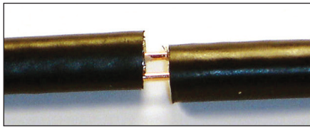
Figure 6 — The final joint with gap of about 1/8 inch. Take care to clear away any wire strands or bits of foil from the center conductors.
