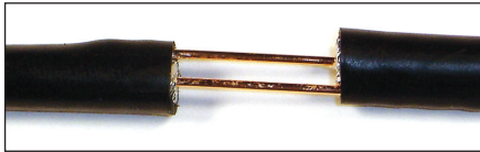
Figure 5 — Continue twisting the two pieces together, keeping the two center conductors parallel.
