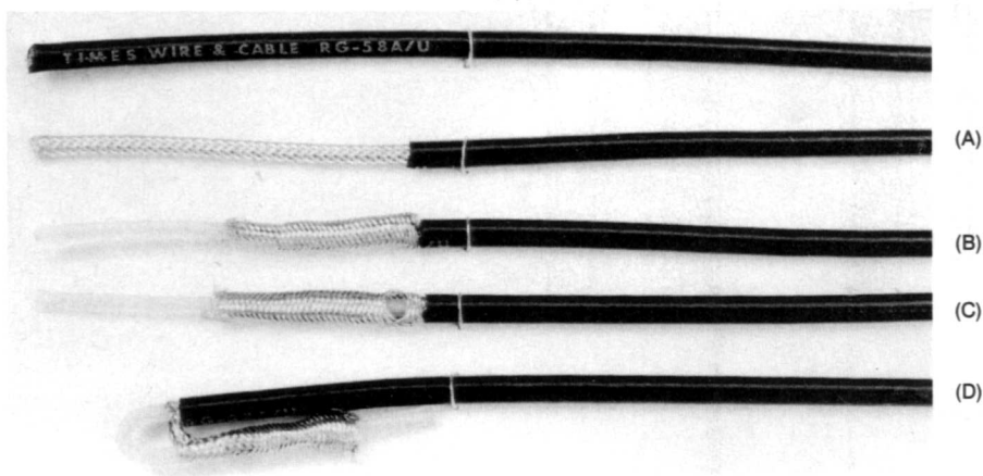
Fig. 3 — The conductors of a coaxial cable can be separated in four easy steps. A — Remove the outer sheath with a knife, being careful not to nick the braid. B — Push the braid accordion fashion against the sheath. C — Make a hole in the braid by separating the strands. D — Bend the cable at the hole and pull the center conductor and dielectric through.
