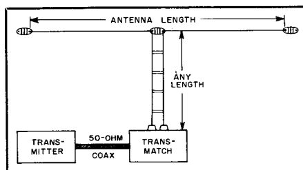
Fig. 2 — This classic antenna is back in vogue because of the widespread use of Transmatches with modern transceivers.
