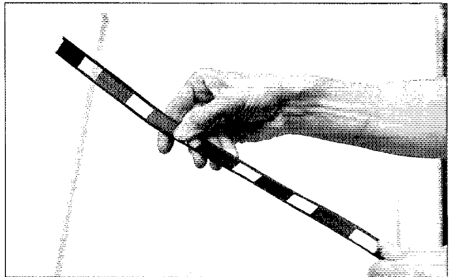
Fig 1—This type of 450-ohm ladder line uses plastic insulating material to maintain a consistent separation between the two conductors. The air gaps between the insulation gives it its ladder-like appearance. Other types of open-wire line are available, but 450-ohm ladder line is the most common.
